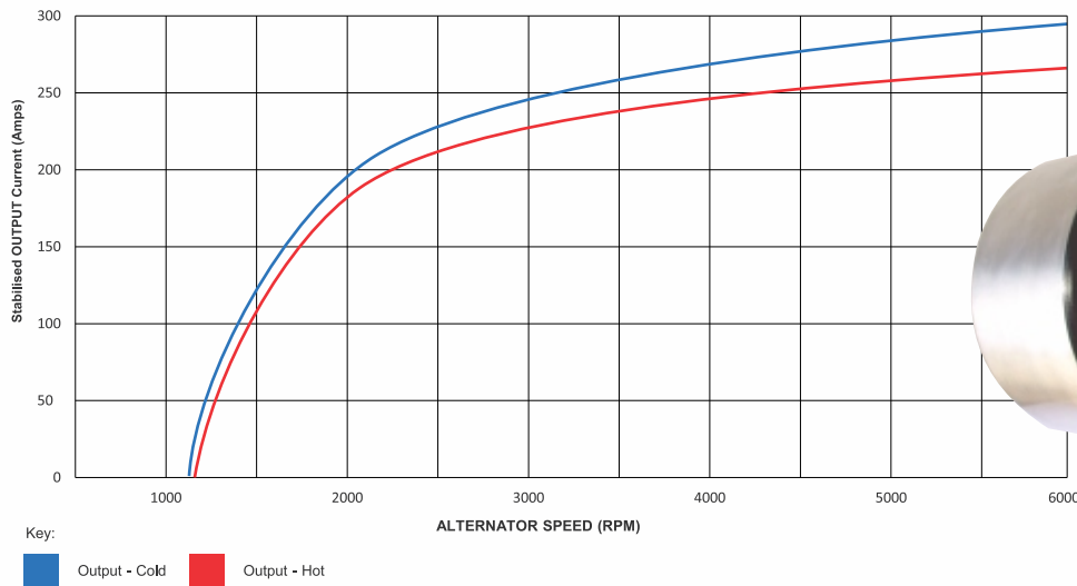
JB26028EMI PERFORMANCE CURVE (@25°C - Ambient measured at 27.0V)
